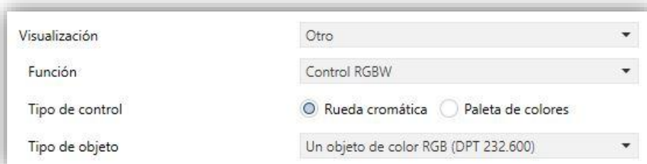
Figura 78. Control RGBW.
