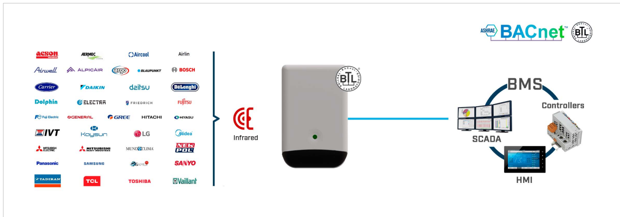
Figure 1. Integration of IR air conditioners into a BACnet installation using the Intesis IN485UNI001/100 gateway
