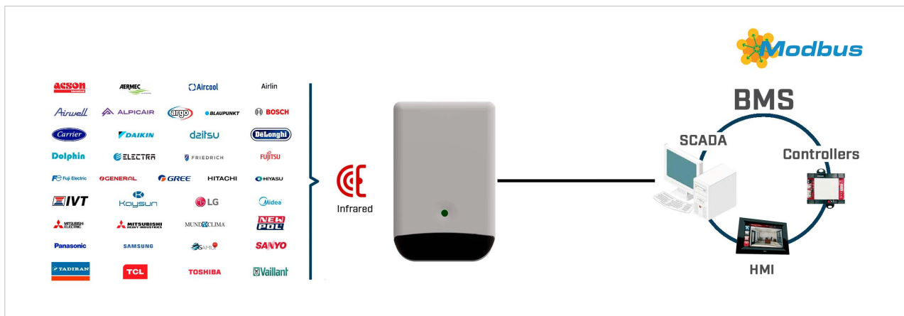
Figure 2. Integration of IR air conditioners into a Modbus installation using the Intesis IN485UNI001/100 gateway
