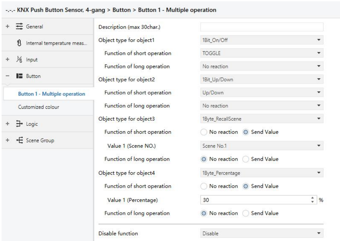
Fig.5.4.10 Parameter setting of multiple operation function
