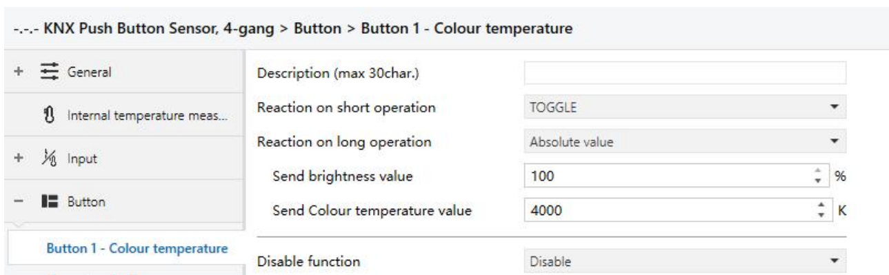
Fig.5.4.5 Parameter setting of colour temperature control function
