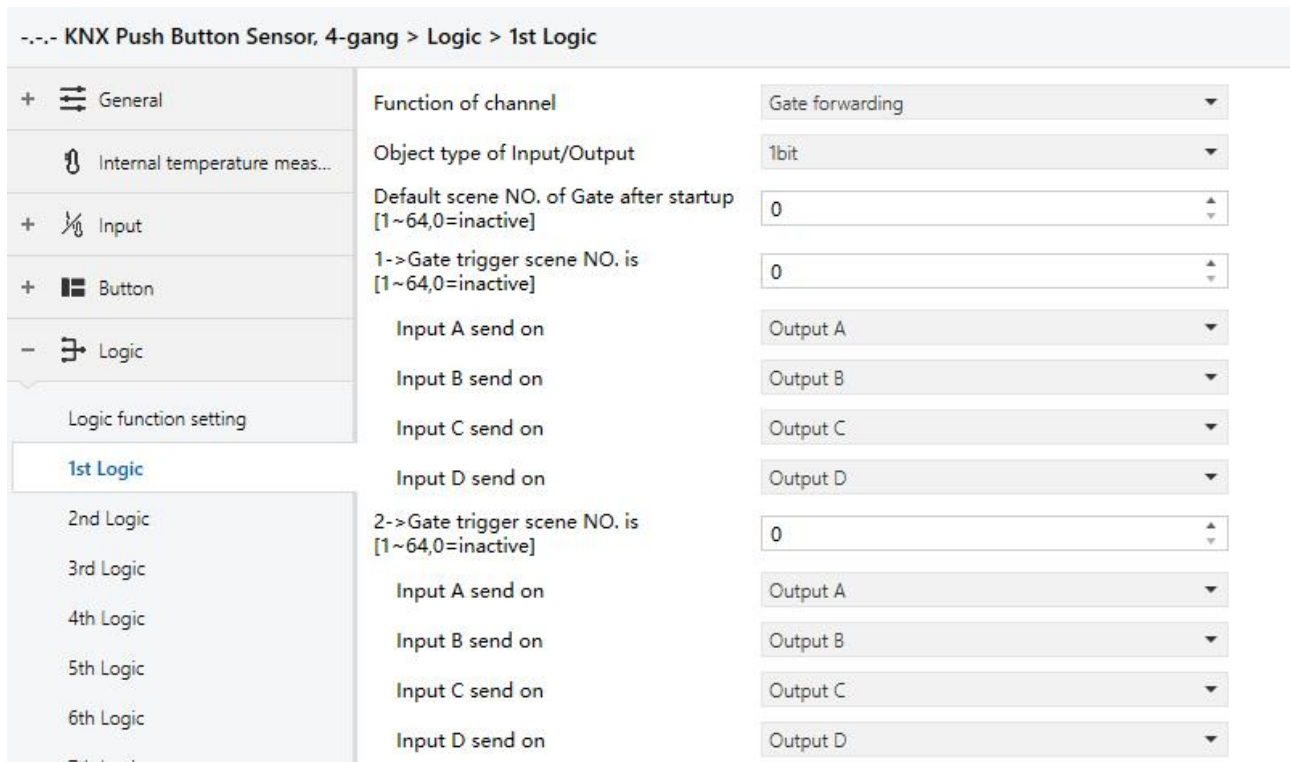
Fig.5.5.2 “Gate forwarding” parameter window
