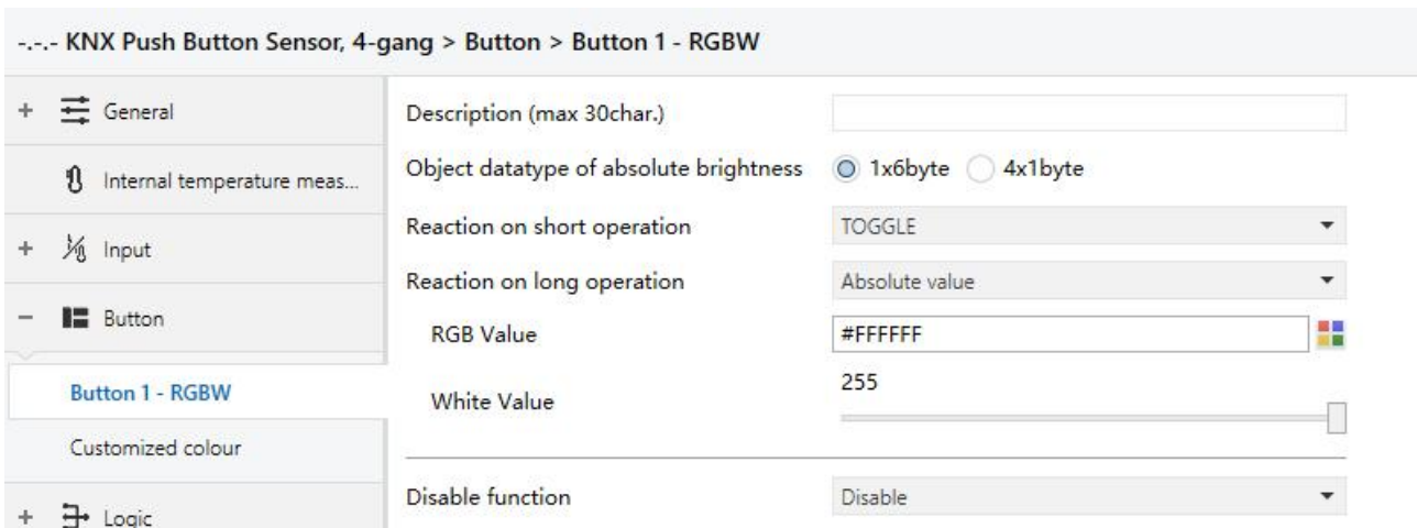
Fig.5.4.4 Parameter setting of RGBW lighting function
