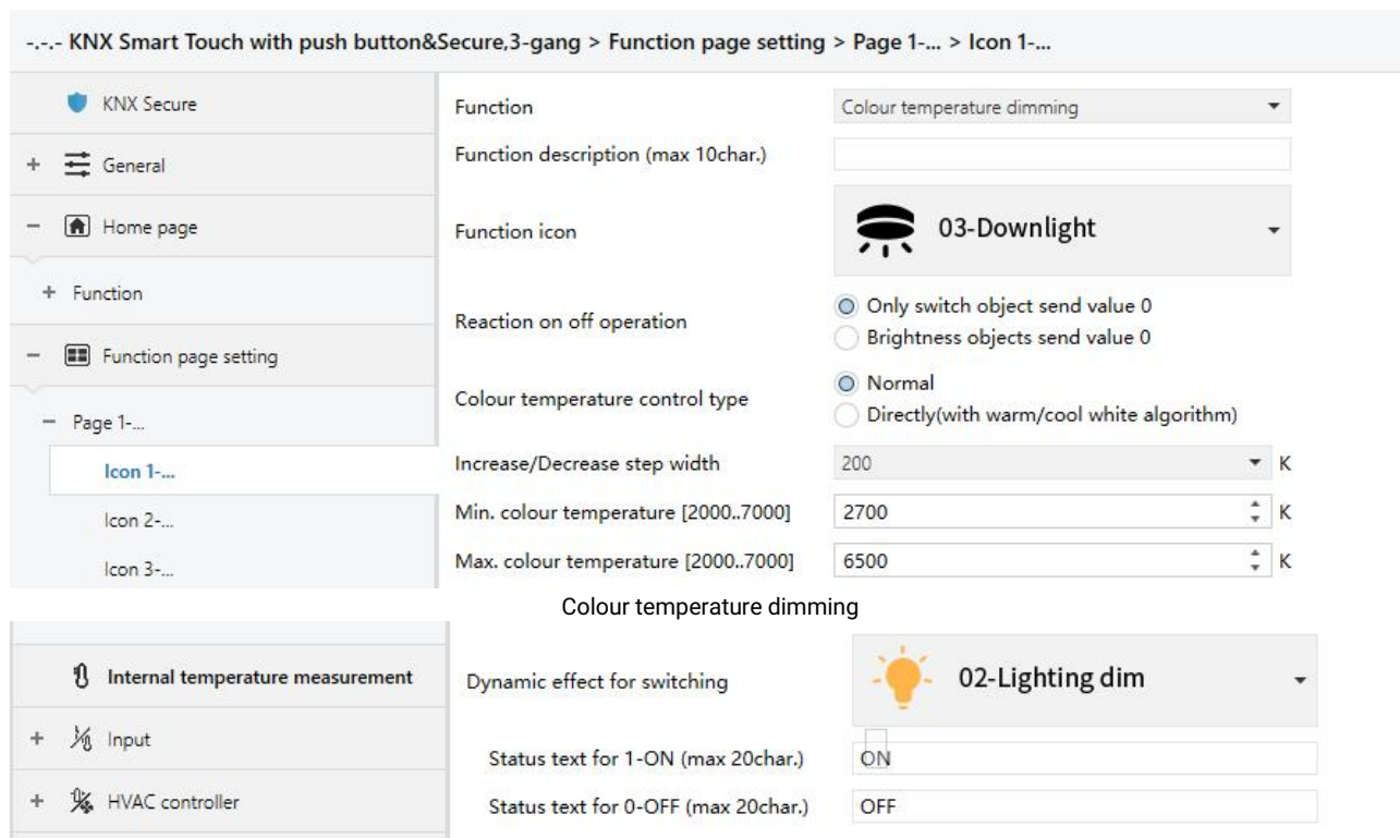
RGB / RGBW / RGBCW / Colour temperature dimming dynamic effect setting Fig.5.7.2.1 (4) Parameter setting of colour and colour temperature dimming function
