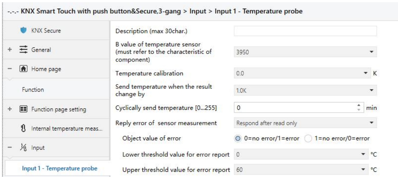
Fig.5.4.1 Parameter setting of temperature probe
