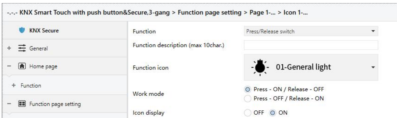
Fig.5.7.2.1 (2) Parameter setting of press/release switch function
