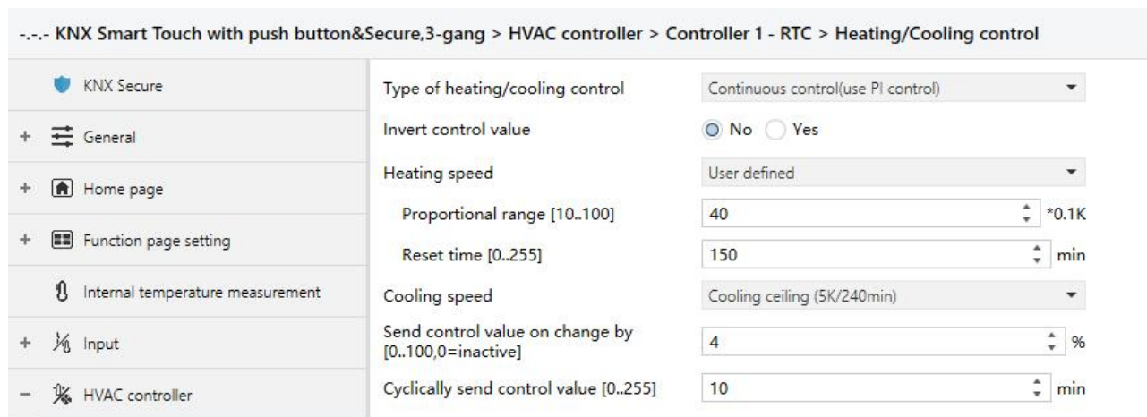
Parameter setting of "Continuous control(use PI control)" Fig.5.5.1.2 "Heating/Cooling control" parameter window
