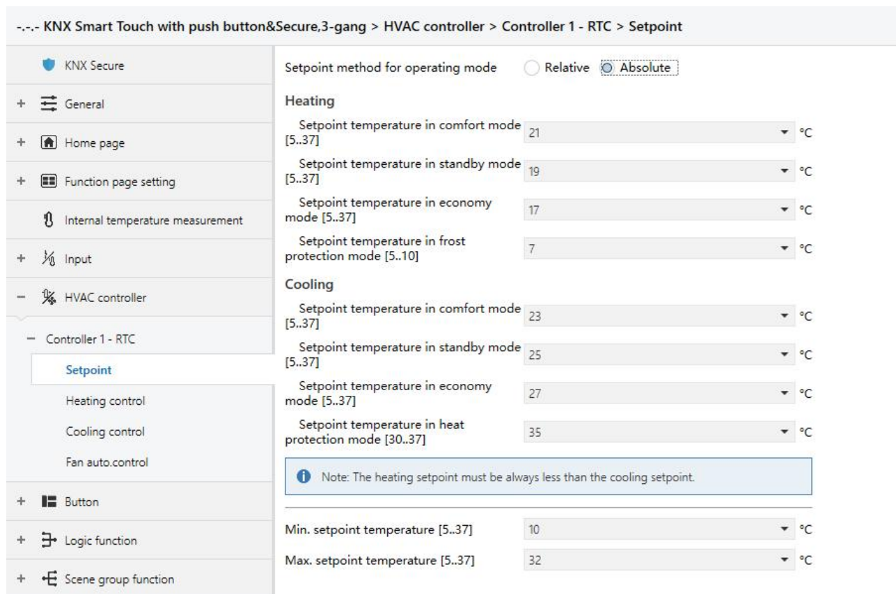
Parameter setting of absolute adjustment
