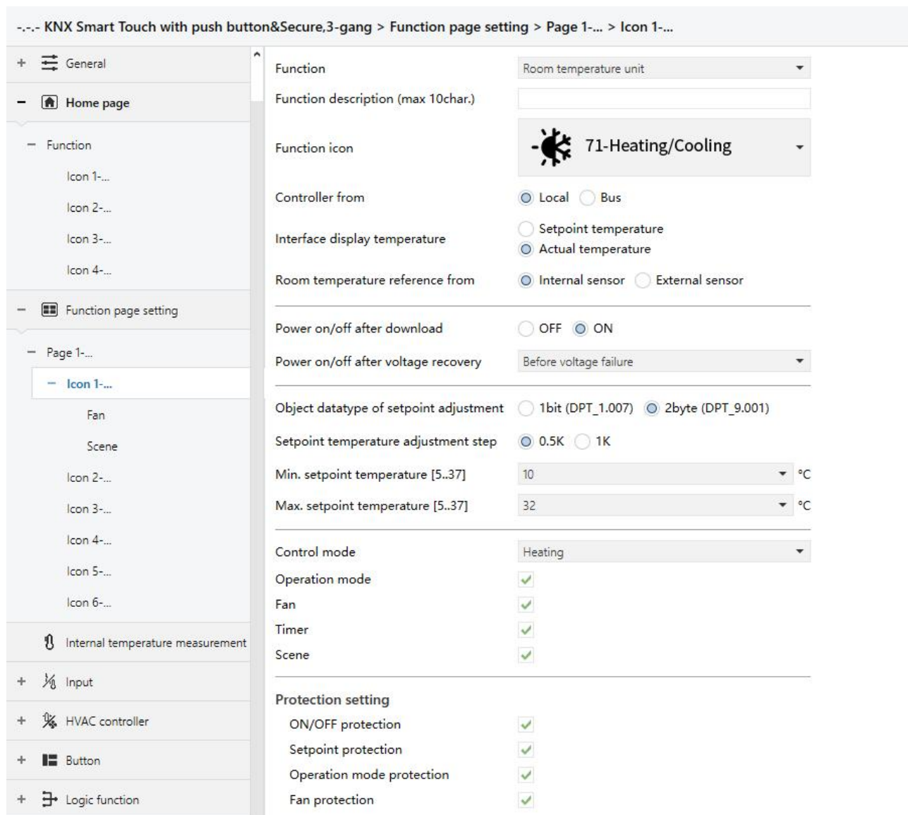
Fig.5.7.2.3(1) room temperature unit function parameter window
