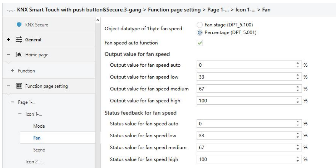
Fig.5.7.2.2(3) Air condition-Fan speed parameter window
