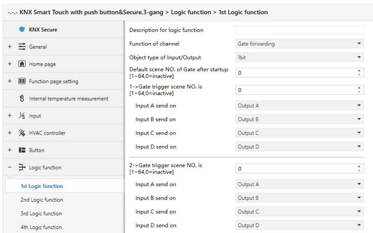
Fig.5.9.2 “Gate forwarding” parameter window
