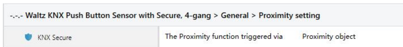
Fig.5.2.2 "Proximity setting" parameter window
